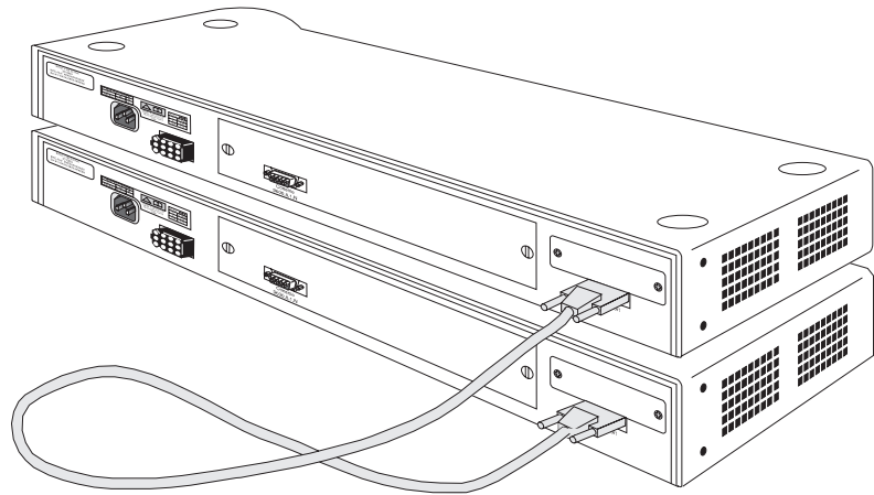
Figure 8 A stack of two units
