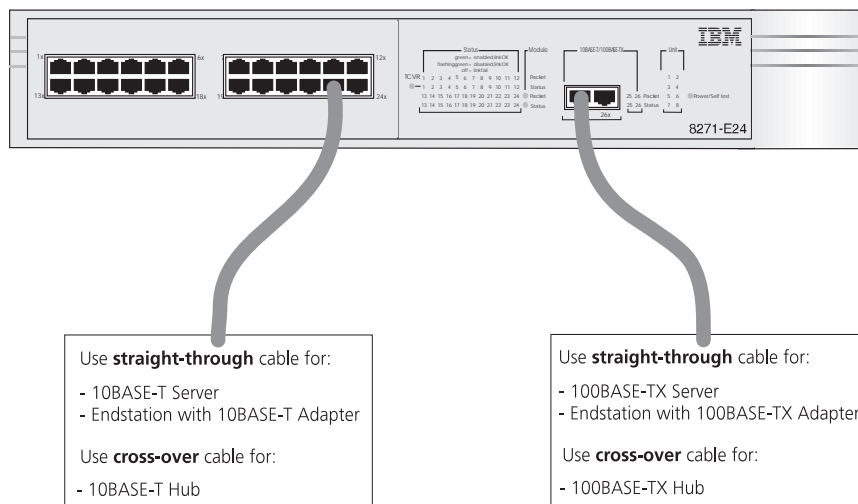
Figure 10 Connecting other devices to the Switch
