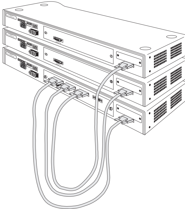
Figure 9 A stack of multiple units
