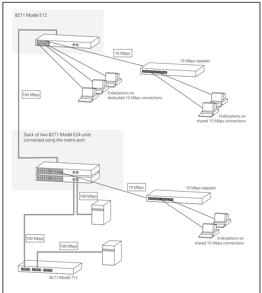
Figure 3 Using the Switch to segment your network
