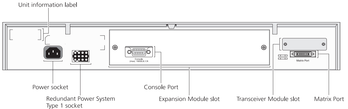
Figure 2 Switch — Rear view
