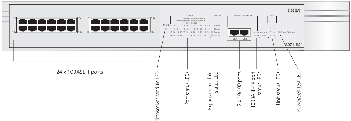
Figure 1 Switch — Front view
