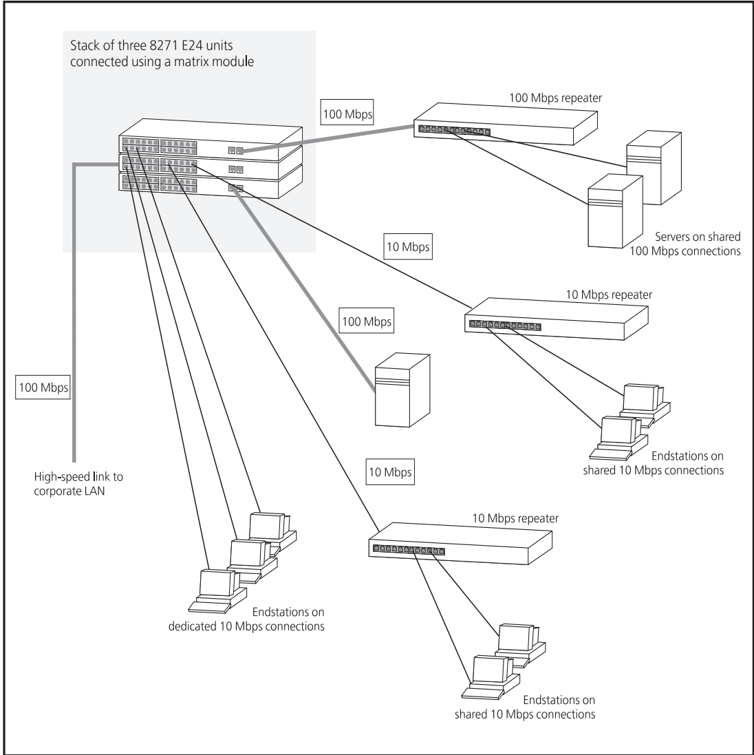
Figure 4 Using the Switch to segment your network
